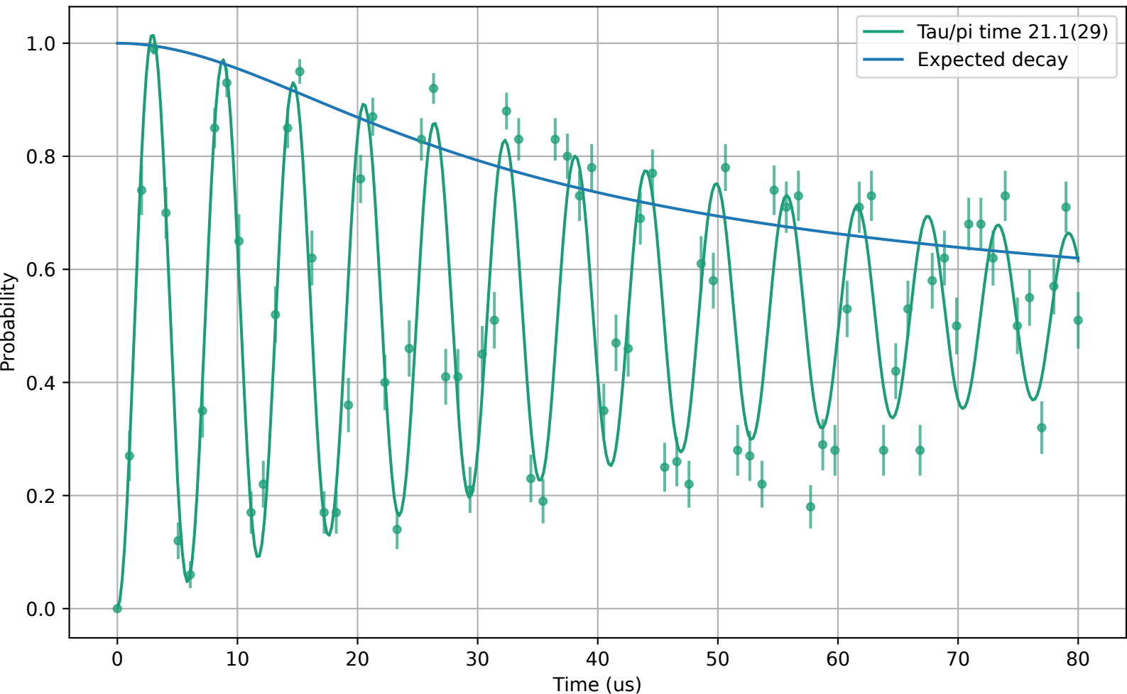
Carrier Flop in 13 Ion Chain
