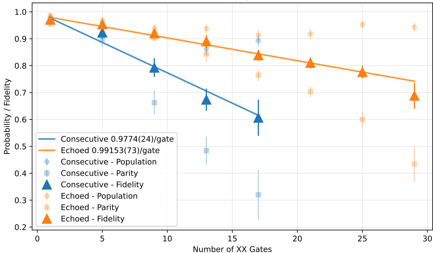
XX Gate Fidelity on -3,4
