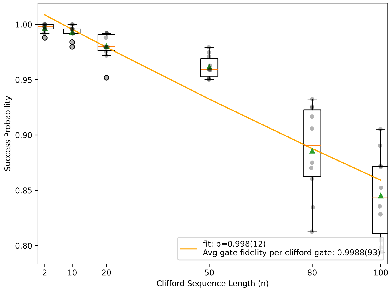
SK1 RB on 13 Ion Chain
