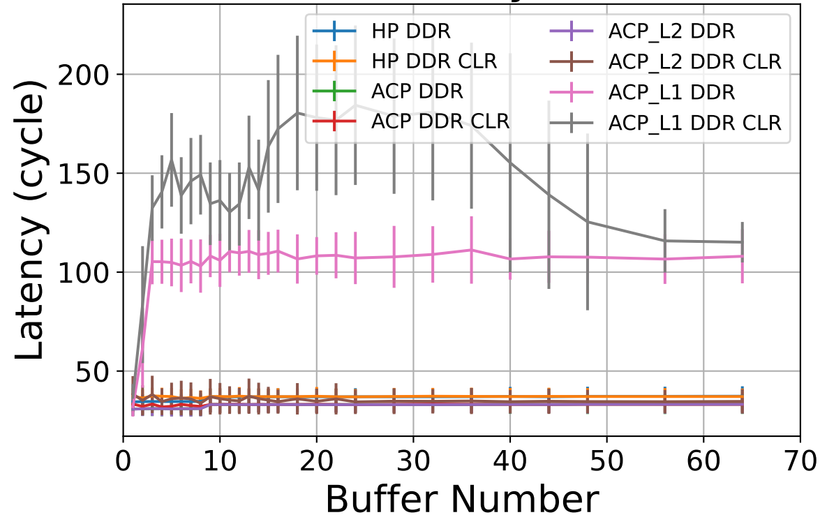
DMA Latency (DDR)
