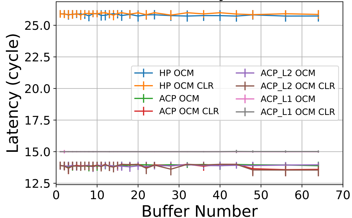
DMA Latency (OCM)
