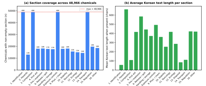
Fig. 4. Per-section coverage of the released dataset over the 16 MSDS sections defined by KOSHA. (a) number of chemicals with non-empty text for each section; sections 1 (chemical/company identification), 3 (composition), 8 (exposure controls), and 14 (transport) are populated for essentially every chemical, while regulatory and physico-chemical detail sections are populated only where the source KOSHA record carries non-placeholder content. (b) average Korean text length per section, conditional on the section being non-empty.
