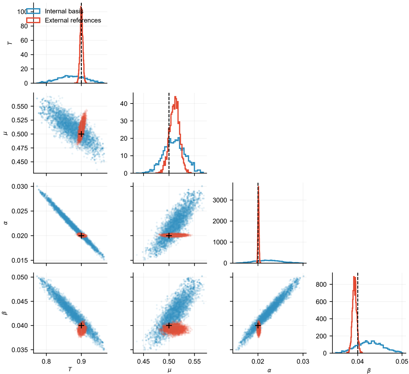
Full four-dimensional bounded posterior
