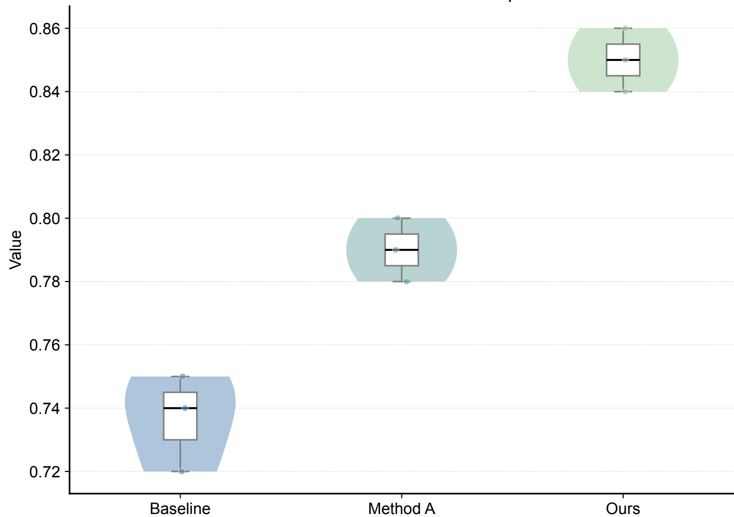
Raincloud Plot: Distribution Comparison
