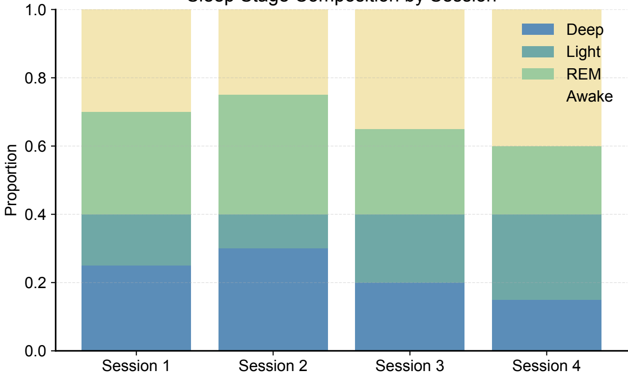
Sleep Stage Composition by Session
