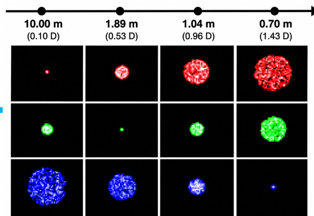
Dioptric-Uniform PSF Allocation
