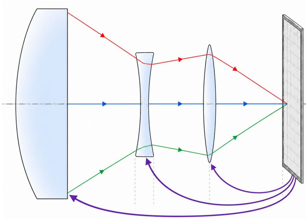
Differentiable Lens Optimization
