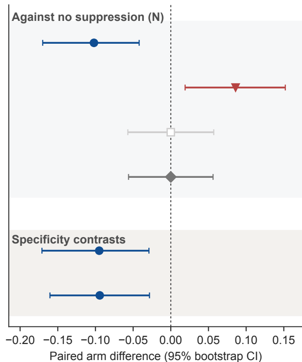
B \Delta permissive RR at B_3
