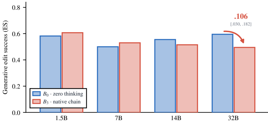
Qwen (R1-distill)
