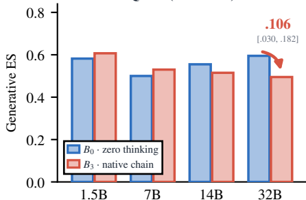
Qwen (R1-distill)
