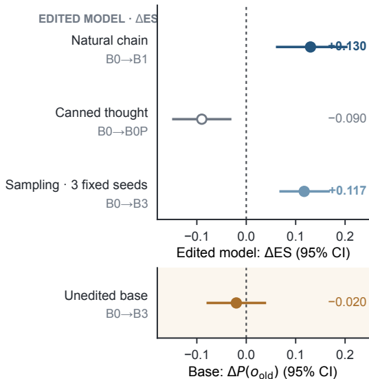
b Qwen-32B controls
