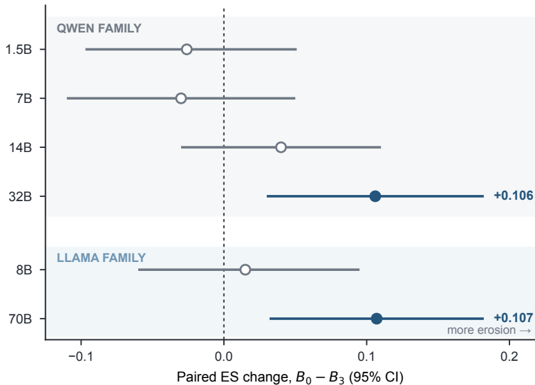
a Paired ES change at fixed checkpoints
