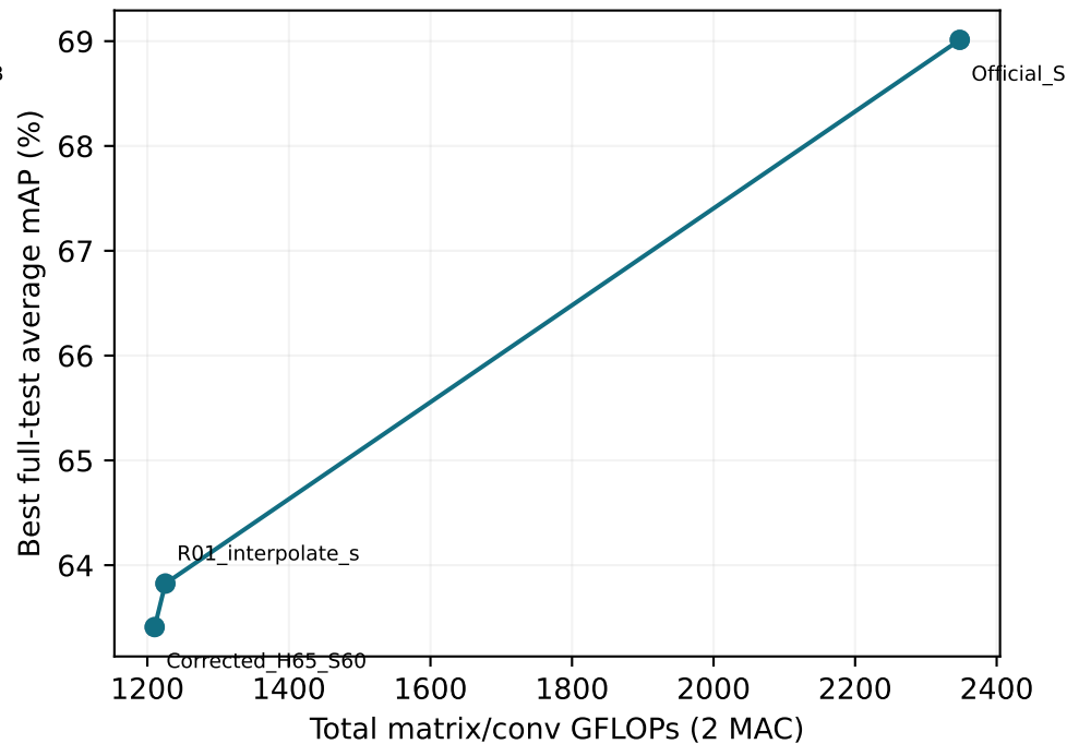
THUMOS14 / VideoMAE-S
