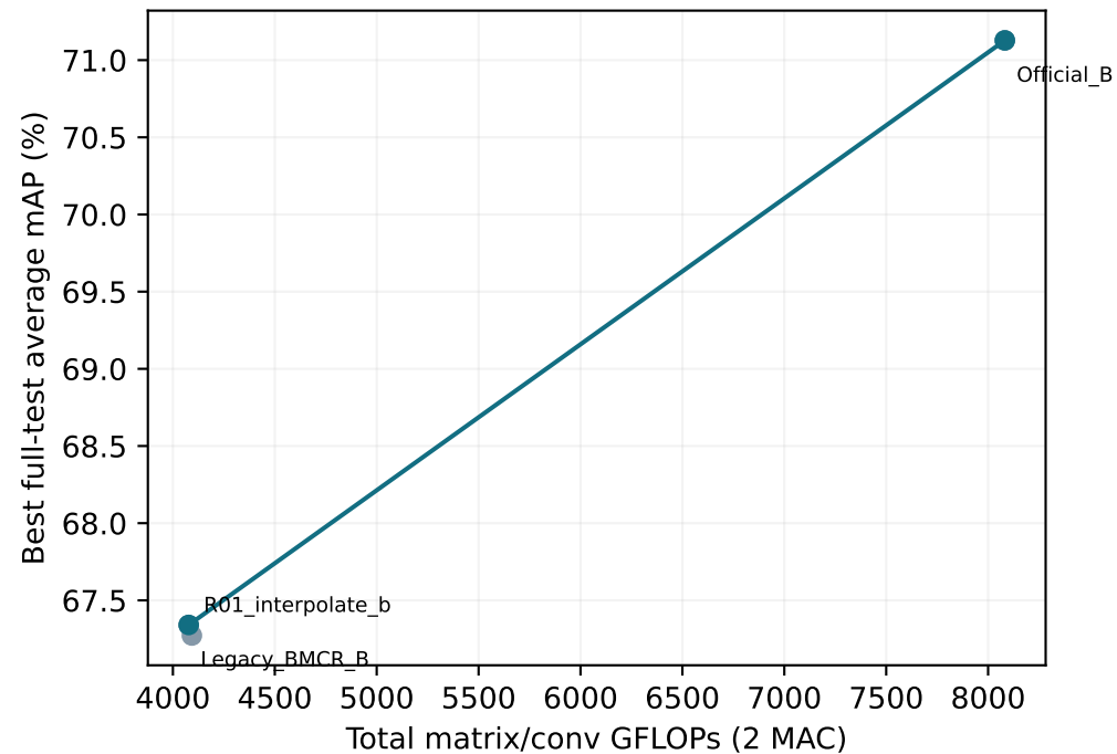
THUMOS14 / VideoMAE-B
