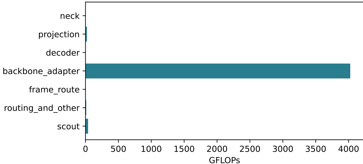
R01_interpolate_b@0_ema
