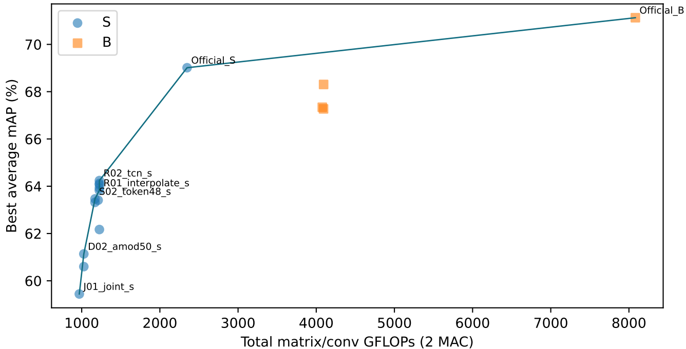
Global model frontier; same dataset and compute scope
