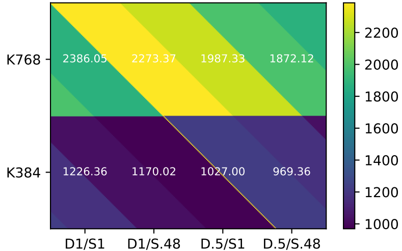
Total GFLOPs
