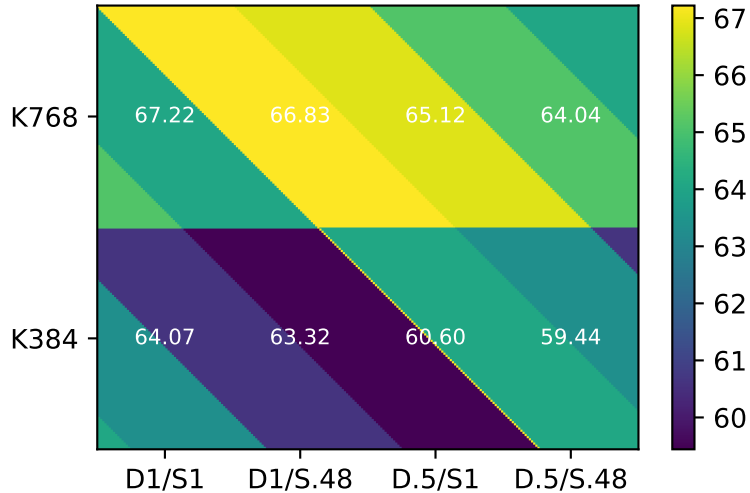
Average mAP (%)
