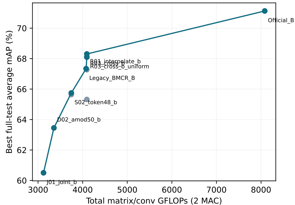
THUMOS14 / VideoMAE-B
