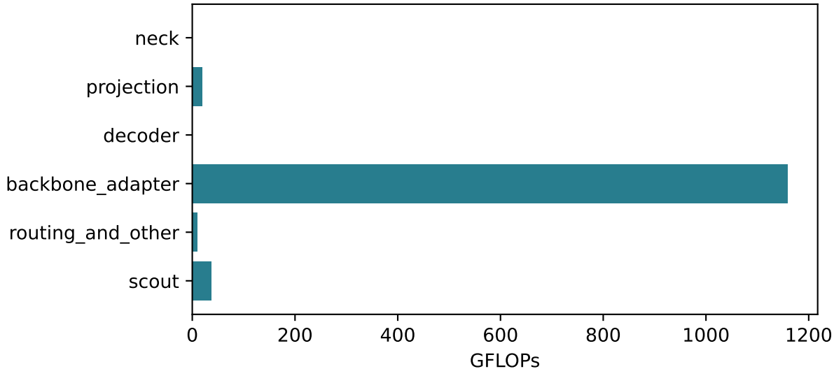
R03_cross_s@5
