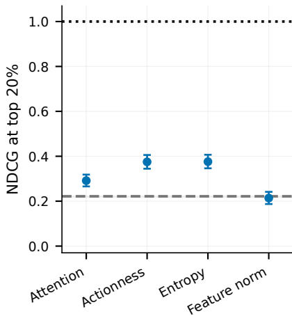
(b) AdaTAD-S / D choices Top-20% relevance
