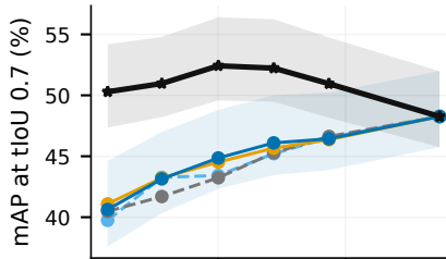
(e) D: Layer-local refinement
