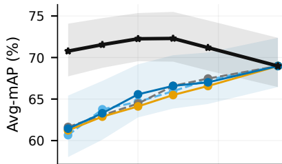
(b) D: Layer-local refinement
