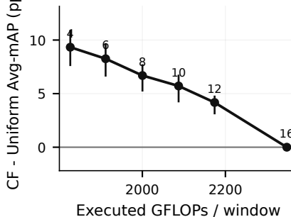
(h) D: paired difference
