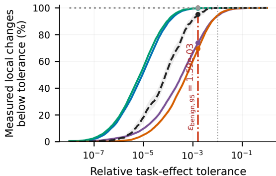
(a) AdaTAD-S: effect magnitude
