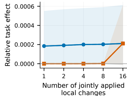
(c) S model / S: joint vs sum
