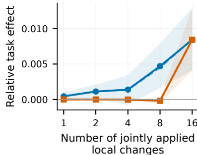
(a) S model / O: joint vs sum
