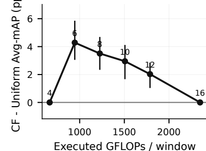
(g) T: paired difference
