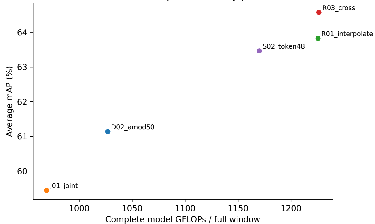
Measured compute-accuracy points
