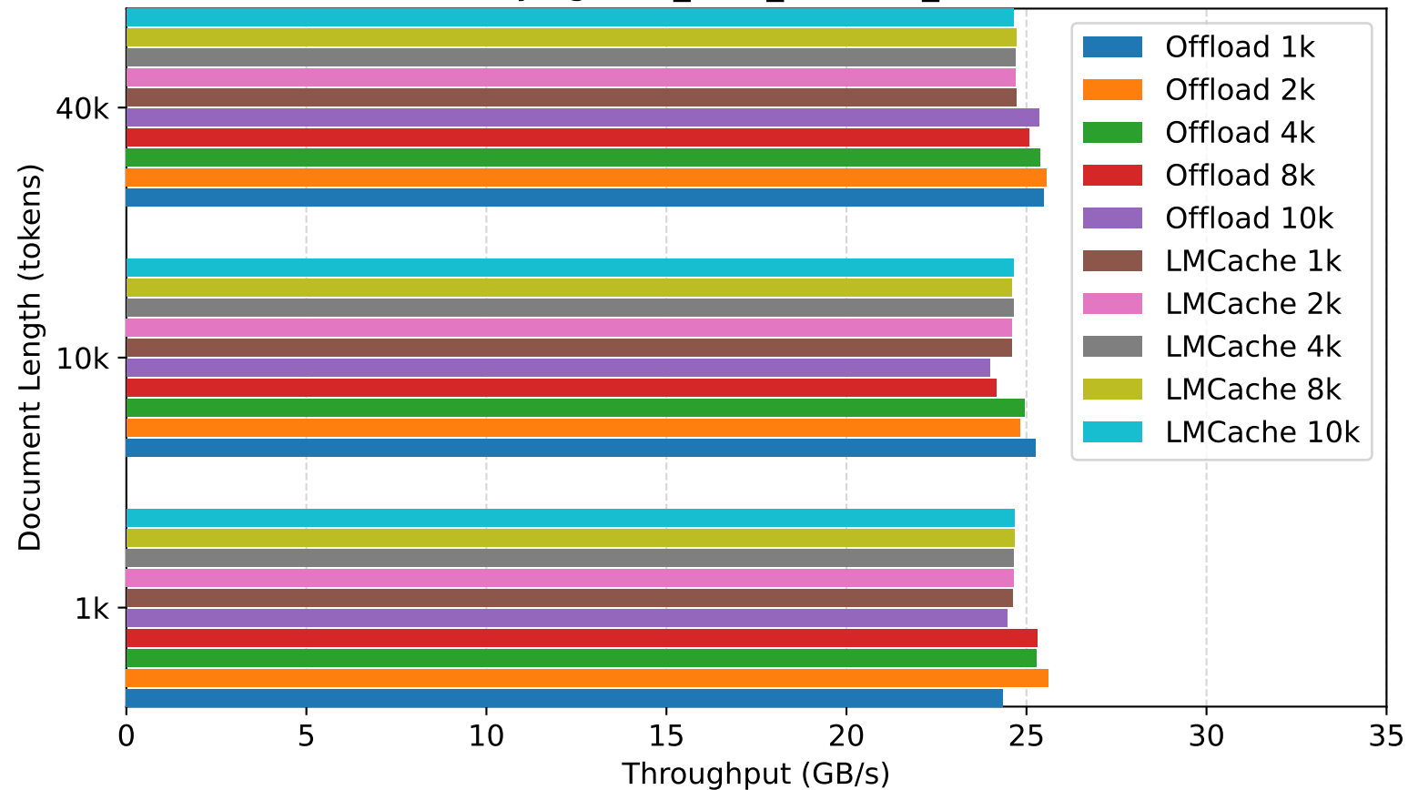
GPU→CPU Transfer Throughput vs Document Length (varying max_num_batched_tokens)
