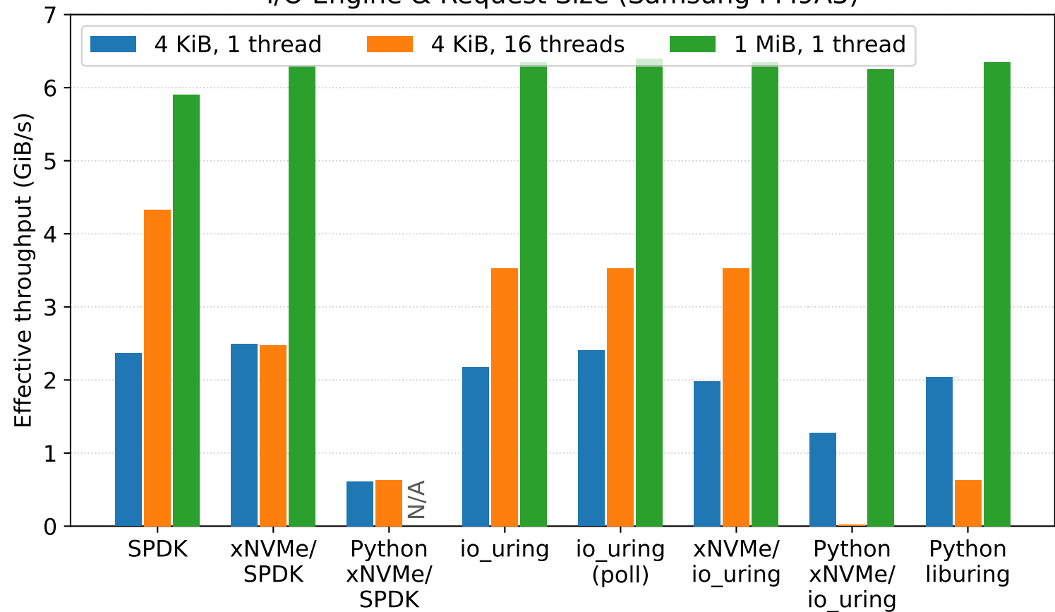
I/O Engine & Request Size (Samsung PM9A3)
