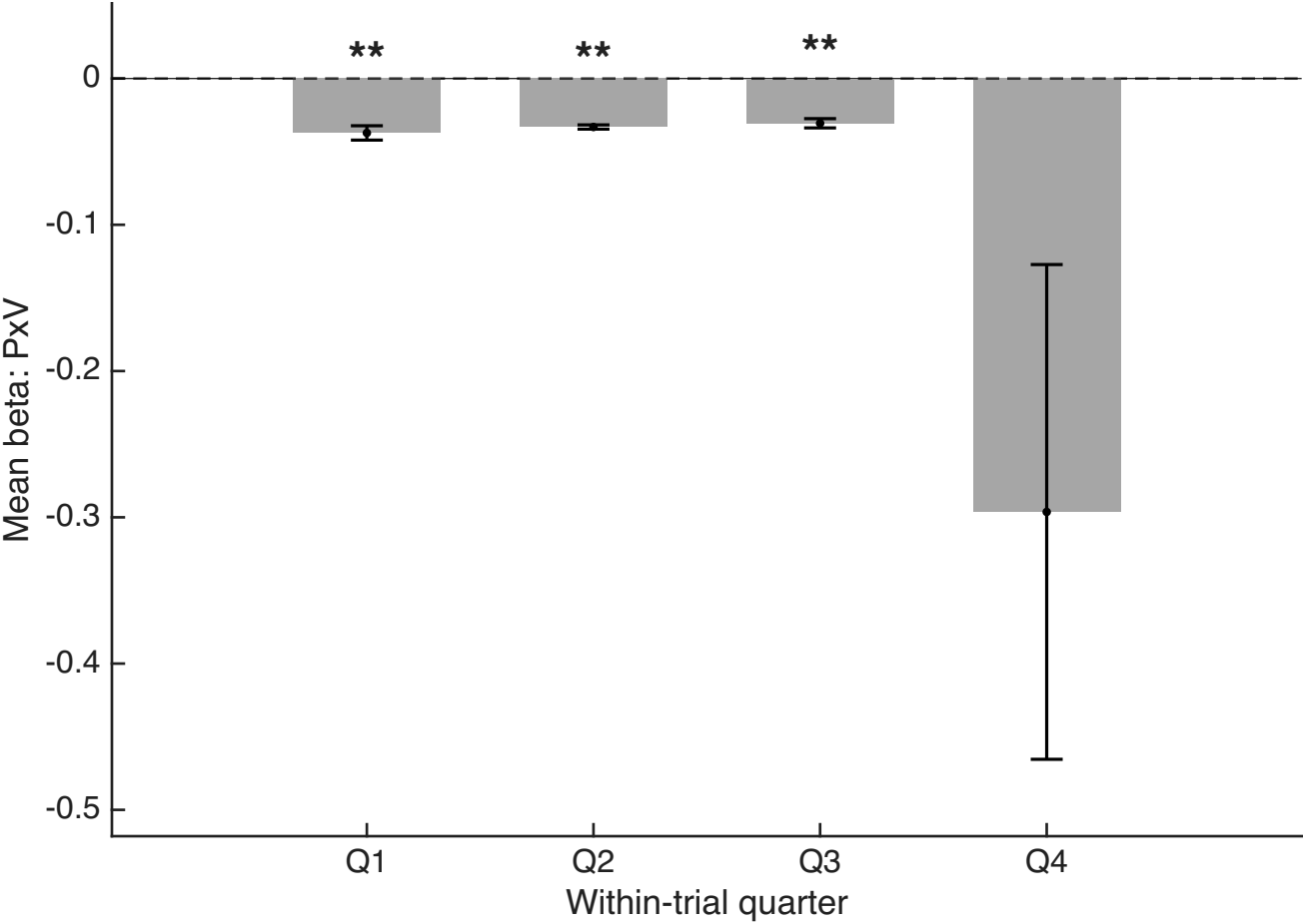
M4_PxV | summary of existing bin betas
