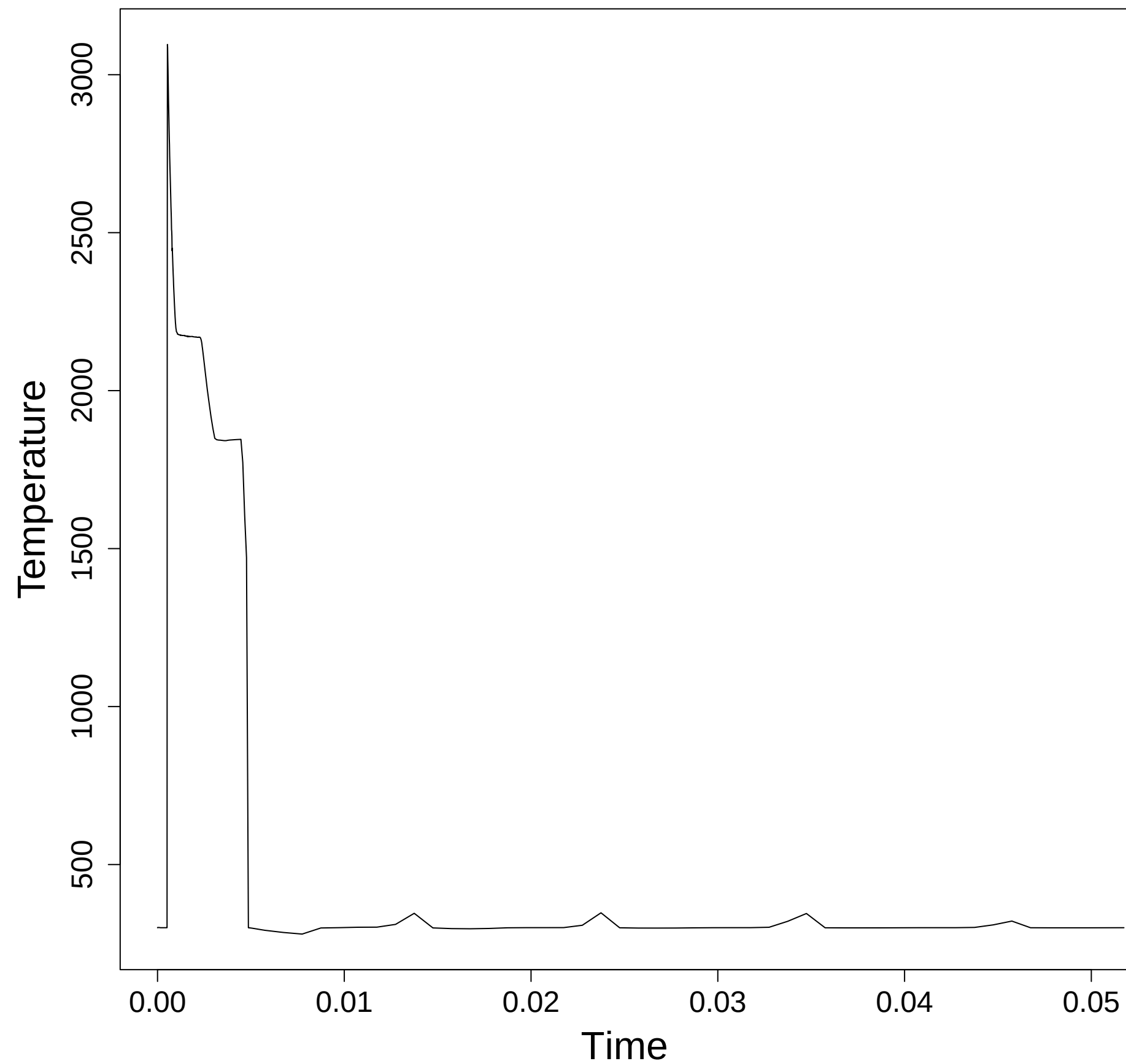
Temperature vs Time
