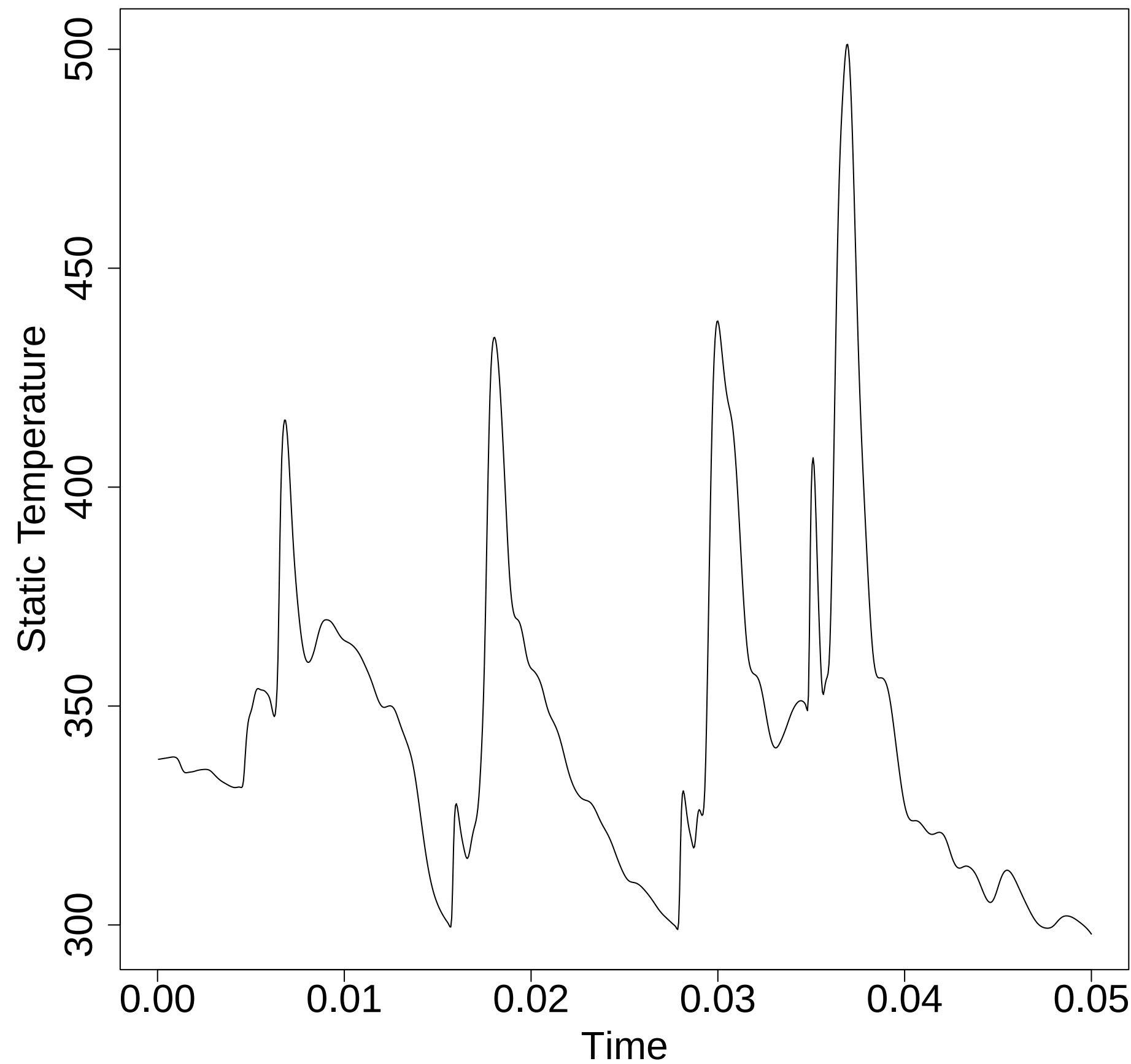
Static Temperature vs Time
