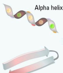
SECONDARY STRUCTURE
