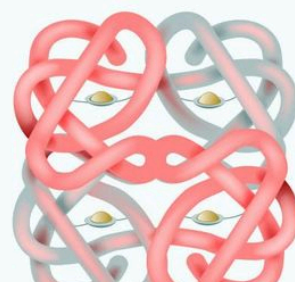
QUATERNARY STRUCTURE
