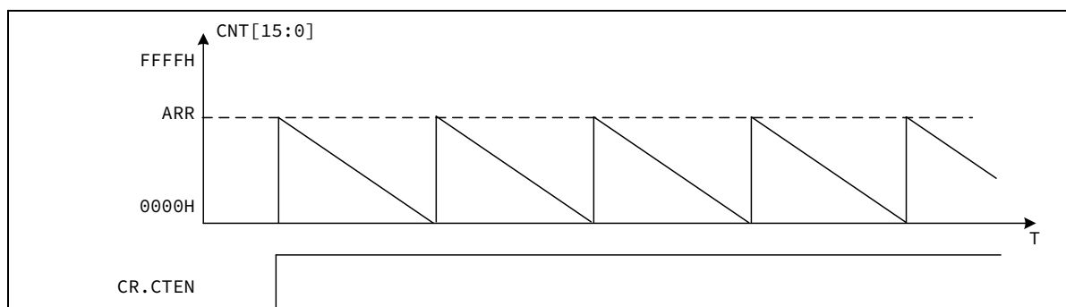
图 13-20 边沿对齐计时器波形 (DIR = 1)
