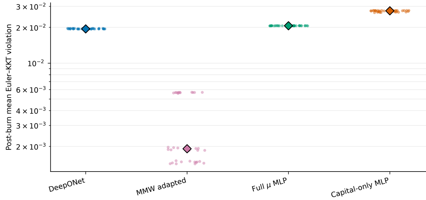
Own-policy paths (diamond: median across 36 paths)
