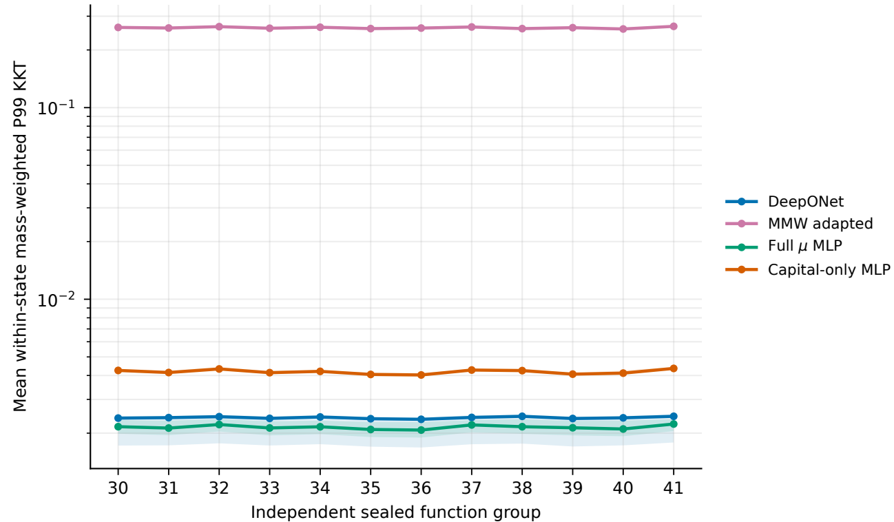
Tail of household equation violations on common states
