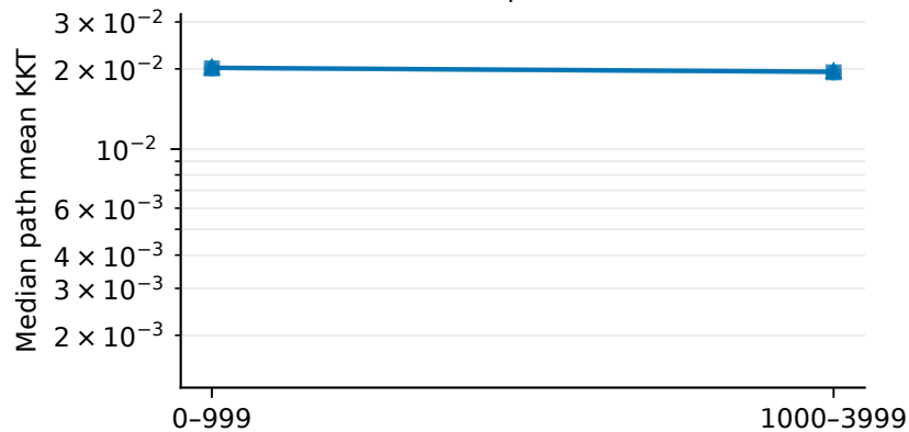
DeepONet
