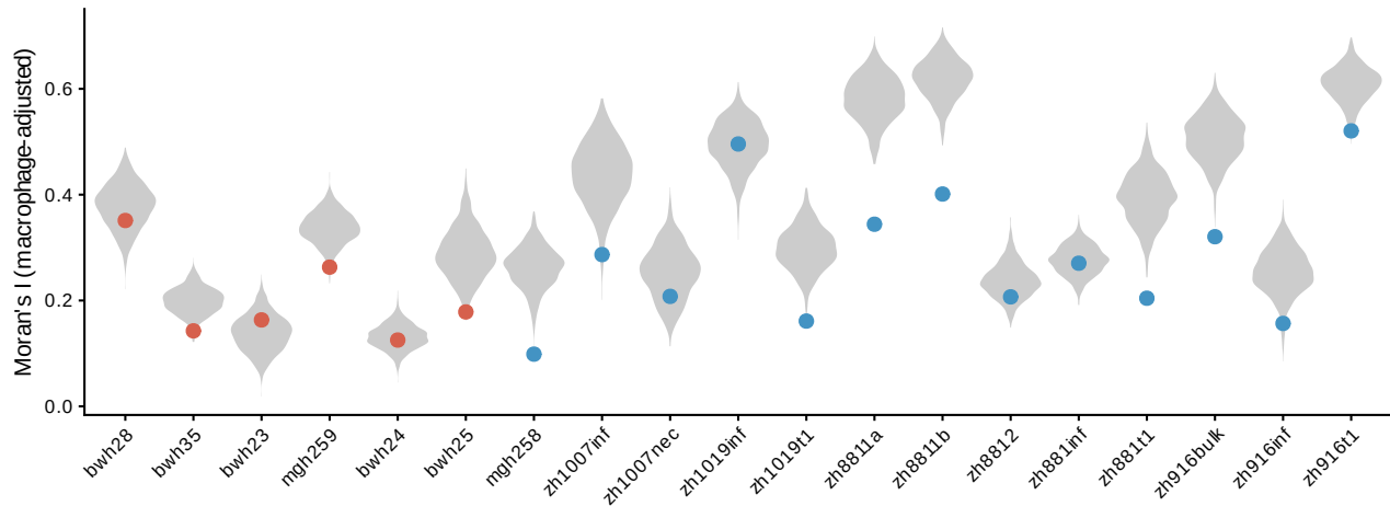
C1b residual after Mac/Inflammatory-Mac MP adjustment
