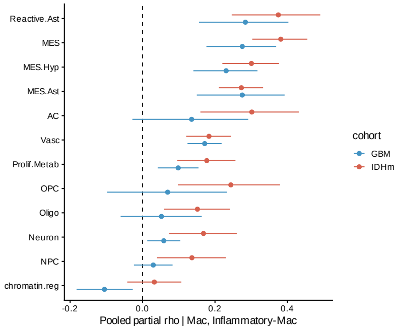
Macrophage-adjusted
