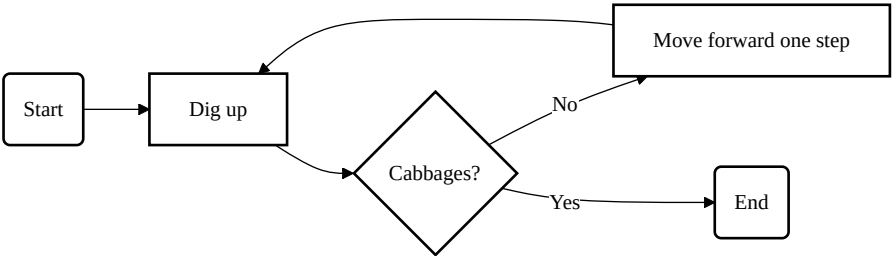
Figure 2: Example Pako
