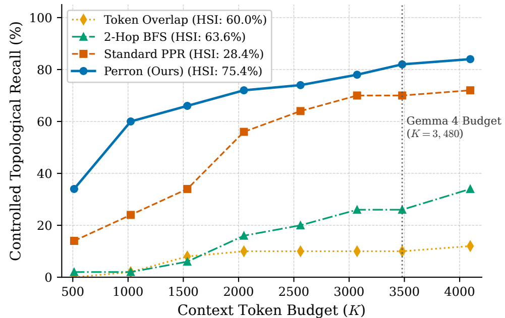
(a) Context Budget Pareto Frontier
