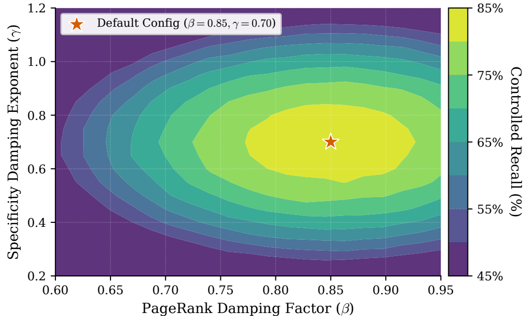
(b) Topological Hyperparameter Sensitivity
