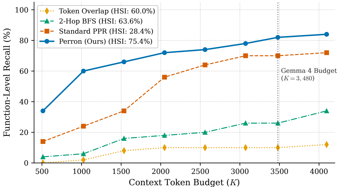
Empirical Pareto Frontier: Context Budget vs. Defect Recall
