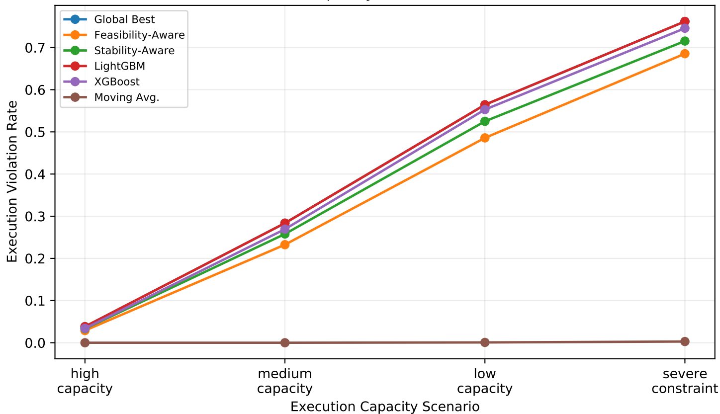
Execution Capacity Versus Violation Rate
