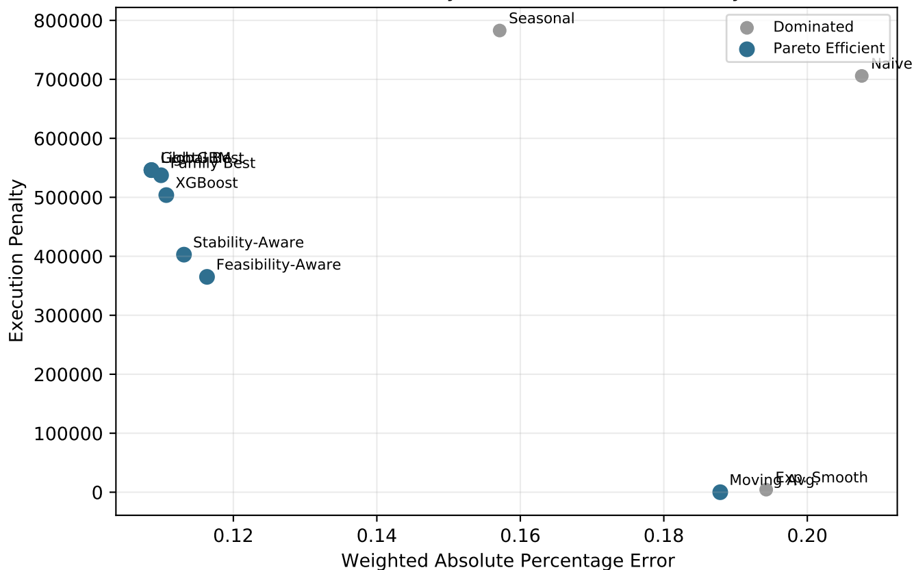
Pareto: Accuracy Versus Execution Penalty
