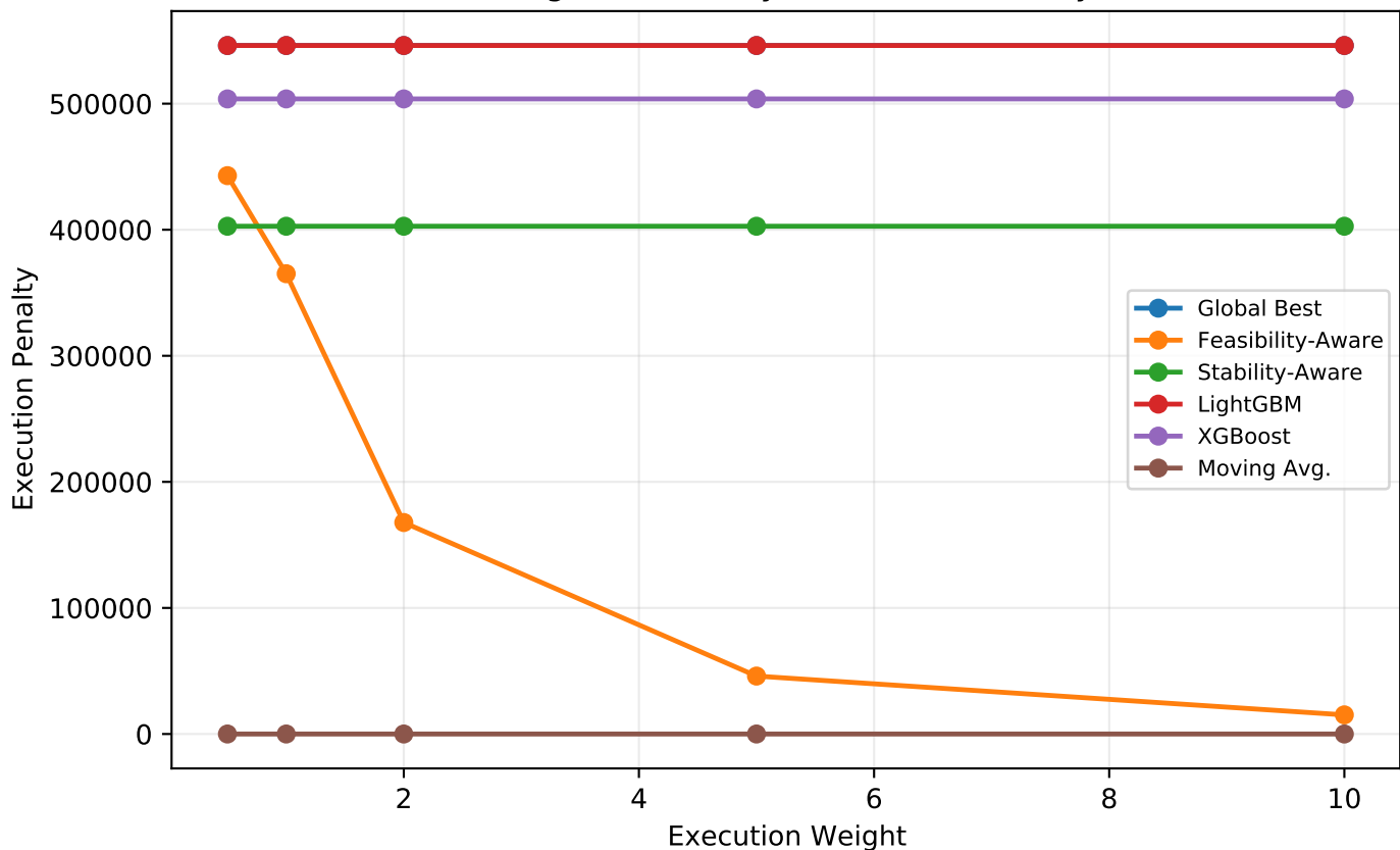
Weight Sensitivity: Execution Penalty
