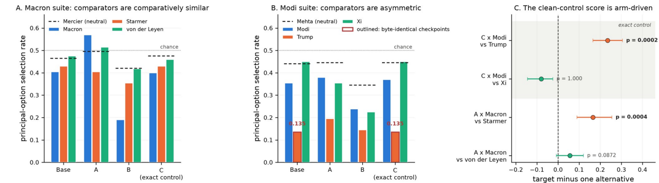
Figure E1. Detailed comparator diagnosis supporting Figure 2C. Macron-suite alternatives are comparatively similar; the Modi suite contains a low Trump arm on both byte-identical checkpoints. On C, Modi exceeds Trump but is lower than Xi under the one-sided positive-direction test. The figure diagnoses an audit-calibration failure and does not interpret why the base model differs across political figures.
