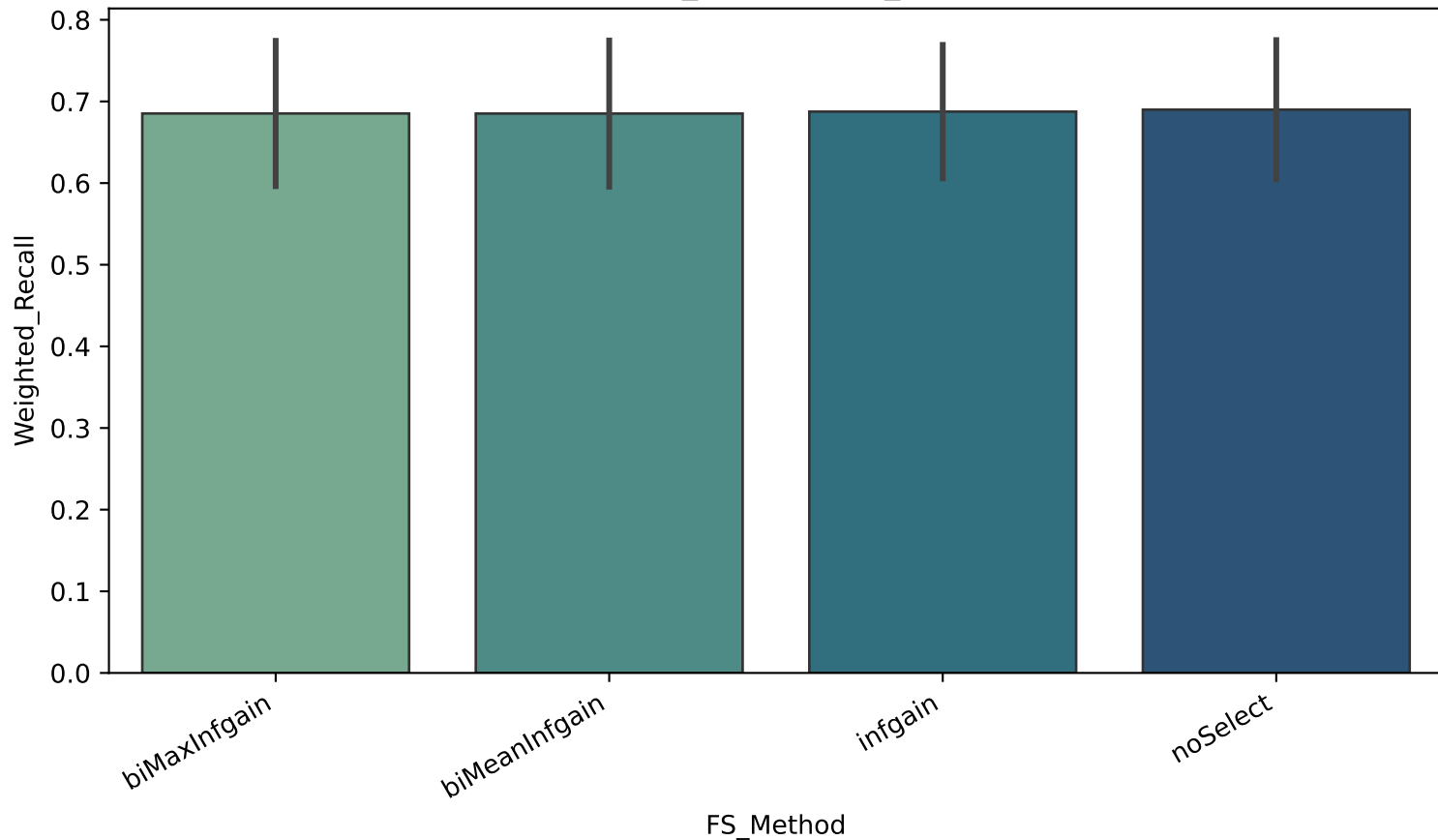
Weighted_Recall by FS_Method
