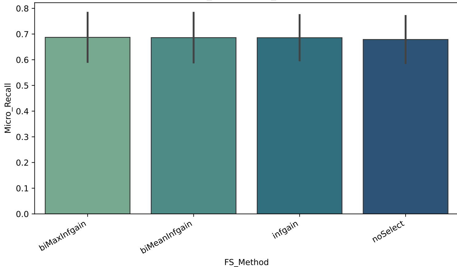
Micro_Recall by FS_Method
