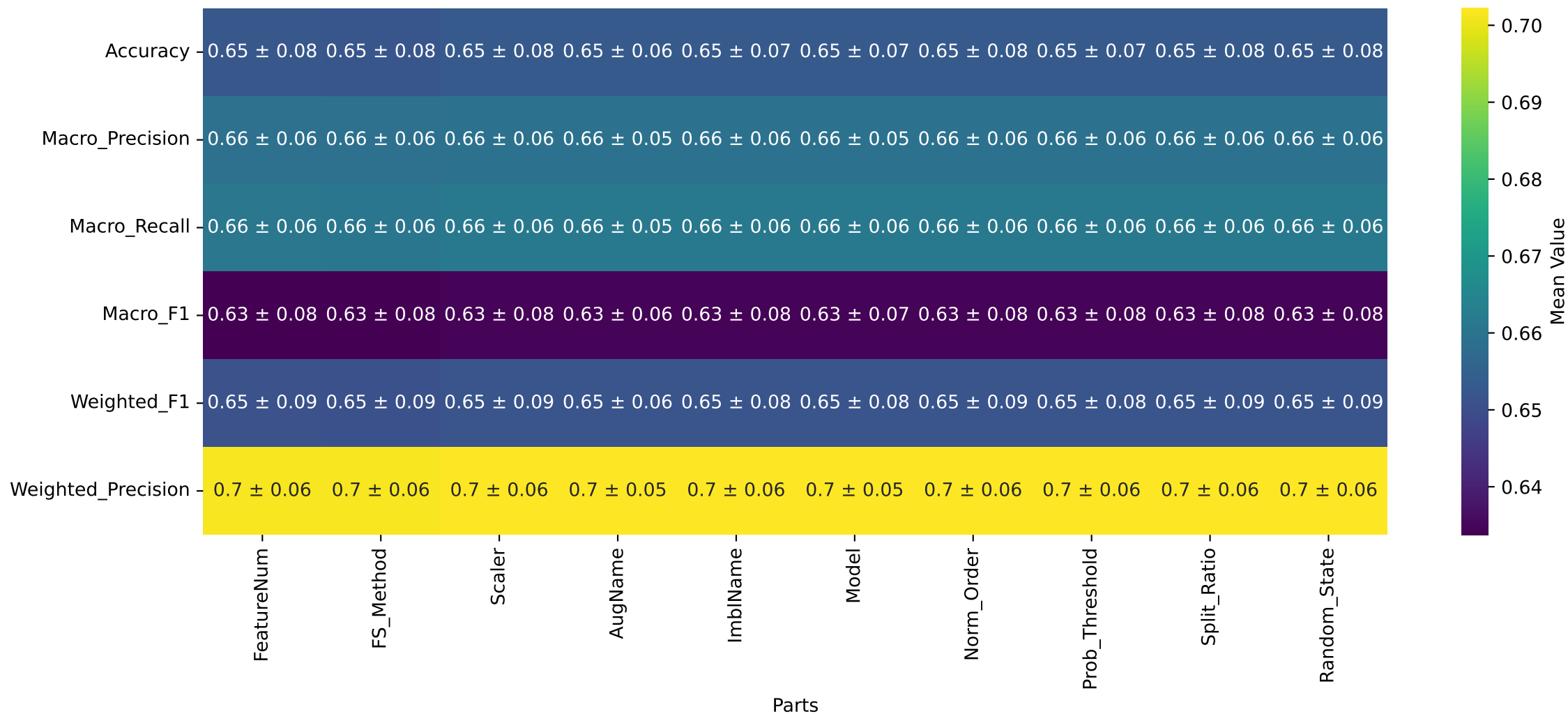
Metrics vs Parts (Mean ± Std)
