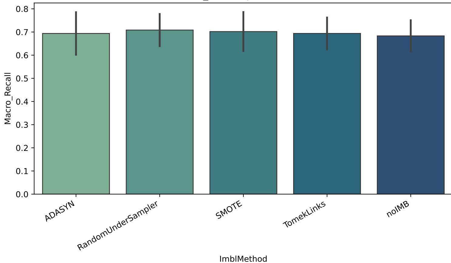
Macro_Recall by ImblMethod
