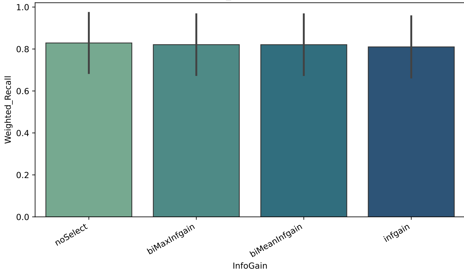
Weighted_Recall by InfoGain
