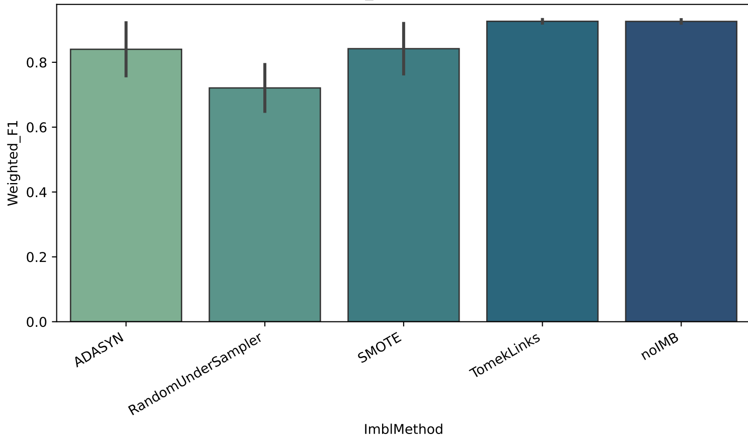
Weighted_F1 by ImblMethod
