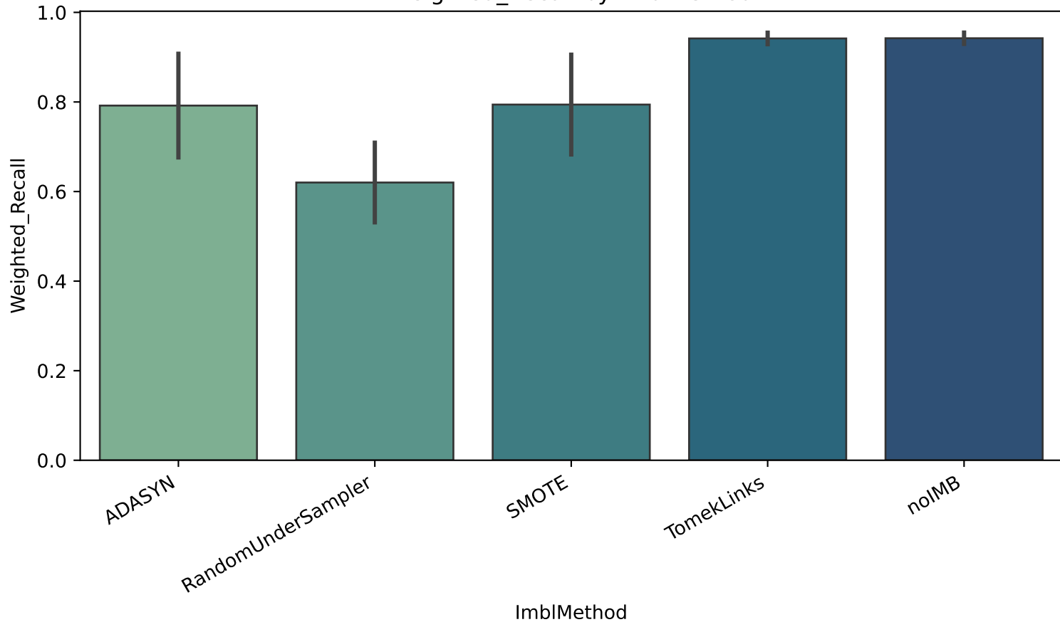
Weighted_Recall by ImblMethod
