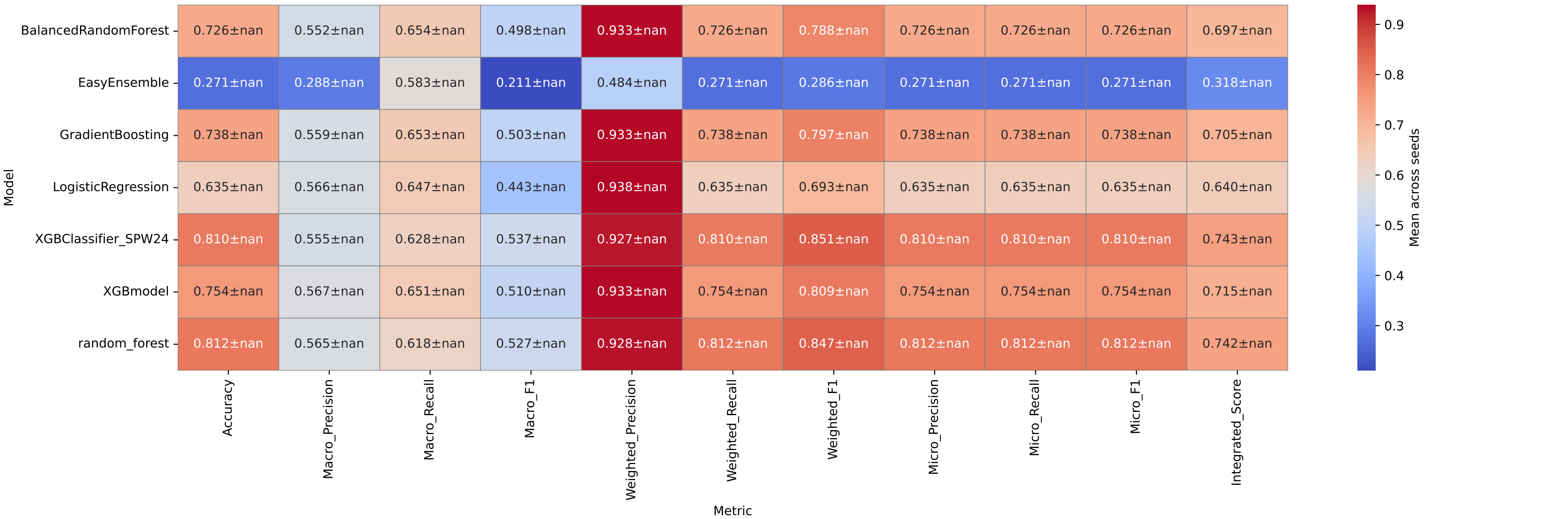
Cross-Seed Performance Deviation (mean ± std)
