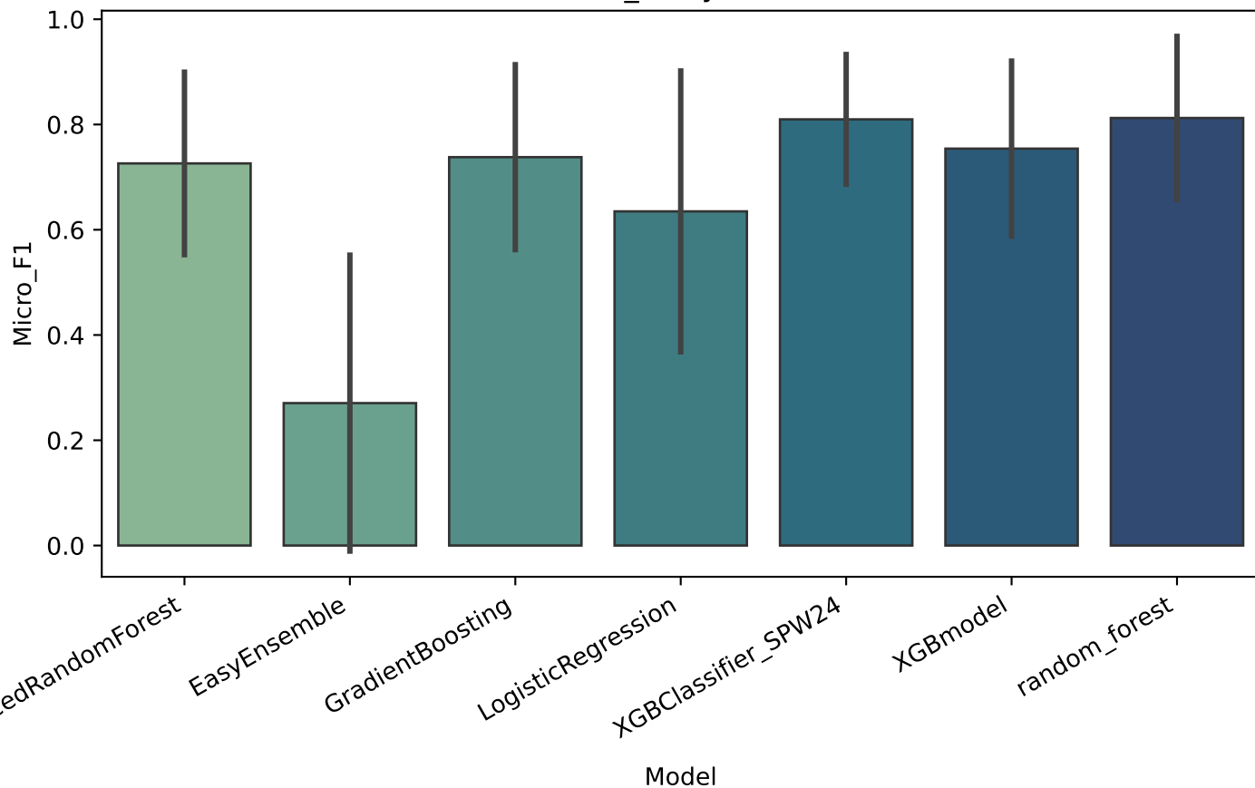
Micro_F1 by Model
